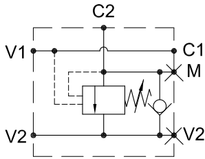
HYDRAULIC DIAGRAM
