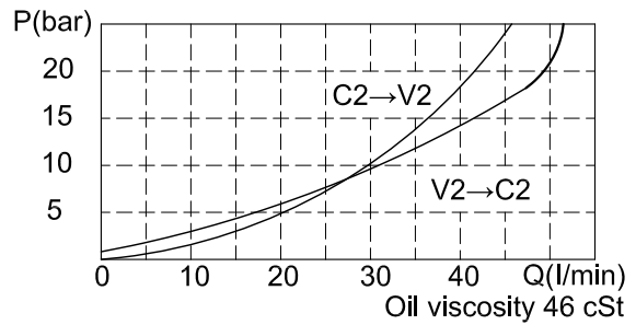
RATING DIAGRAM
