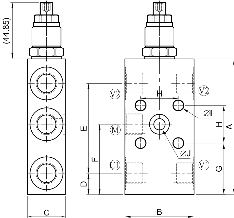
DIMENSIONS ( mm )
