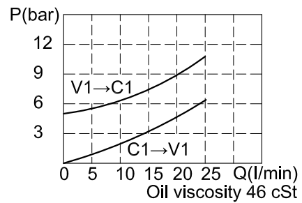
RATING DIAGRAM
