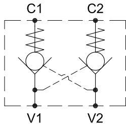
HYDRAULIC DIAGRAM
