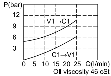
RATING DIAGRAM
