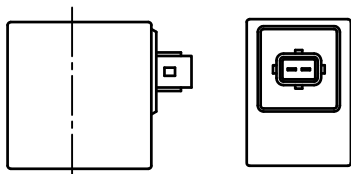
D16-03-12-28 Connection=AMP Junior connection AMP初级电磁线圈
