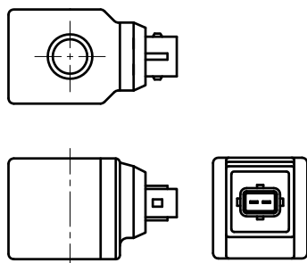
D13-03-24-26 Connection=AMP Junior connection AMP初级电磁线圈
