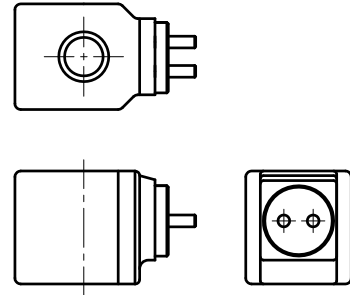
D13-04-24-26 Connection=M27x1 connection M27x1电磁线圈
