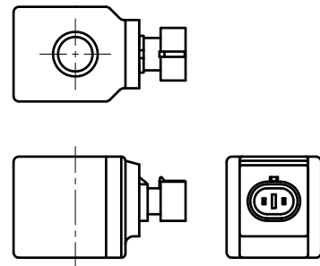
D13-06-24-26 Connection=AMP super seal connection AMP超级密封电磁线圈
