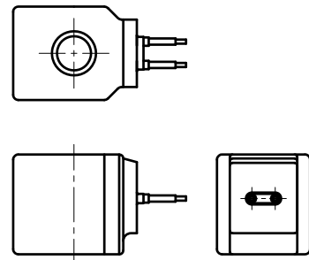
D13-02-24-26 Connection=Lead wires connection 出线型电磁线圈
