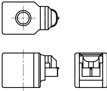
D13-07-24-26 Connection=AMP super seal connection AMP超级密封电磁线圈
