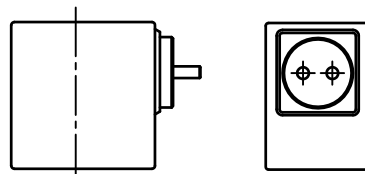
D16-04-12-28 Connection=M27x1 connection M27x1电磁线圈
